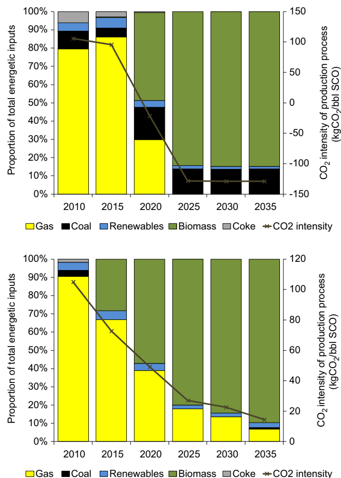
Fig. 6. Energy inputs and carbon intensity of synthetic crude oil production in Canada by in situ means in LCS (top) and LCS-noCCS (bottom).
